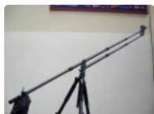
Lot: 651 JIB, Carbon Fibre – Very light weight. Extended length: 2m, max Load: 4kg, Folded 80cm. Net weight: 1.8kg. Contents: Front + Rear section with Brackets and Carry bag.
